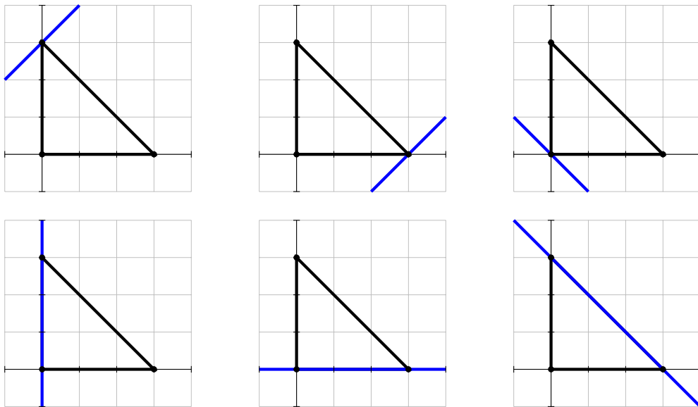
Figure 2.2: A supporting hyperplane for each nontrivial face of the triangle in Figure 2.1
